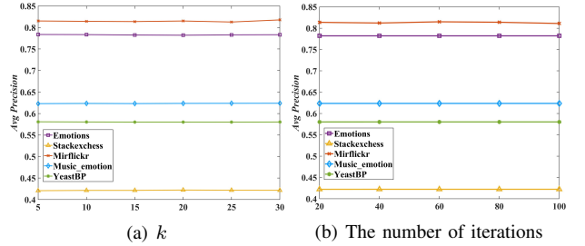
Fig. 6. The Avg Precision results of PML-WFGALC with varying values of k and the number of iterations on various datasets.
