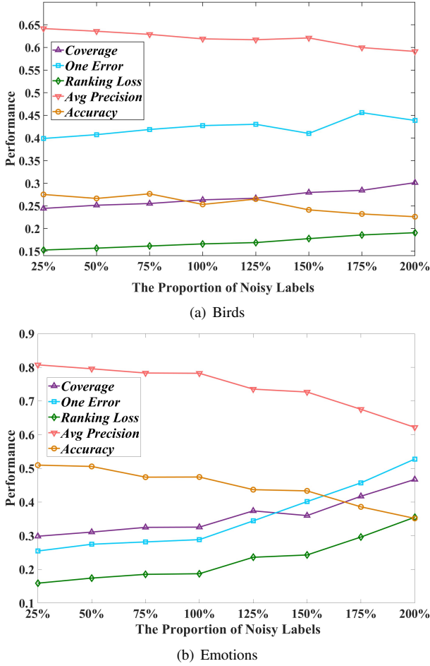
Fig. 4. Robustness analysis of the performance when the proportion of noise in Birds and Emotions datasets is varied.
