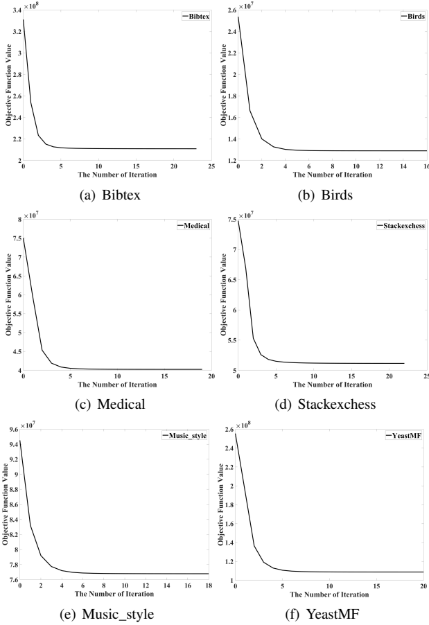
Fig. 7. Convergence curves of PML-WFGALC on six datasets.
