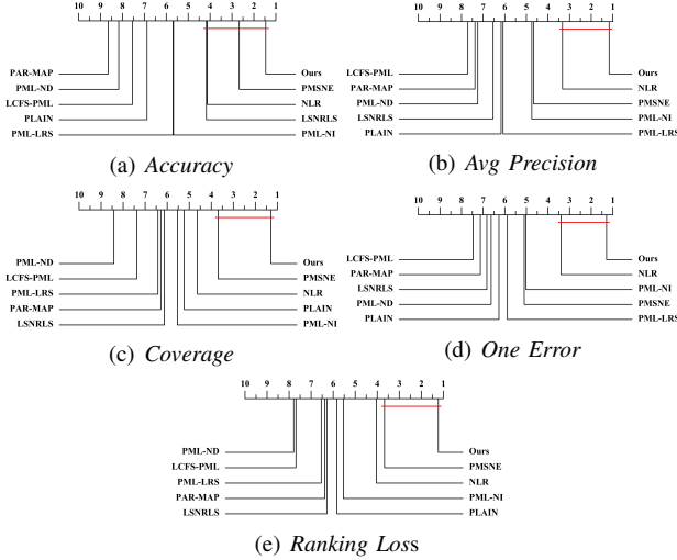
Fig. 3. Comparison of our approach (control algorithm) against nine comparative baselines with the Nemenyi test.
