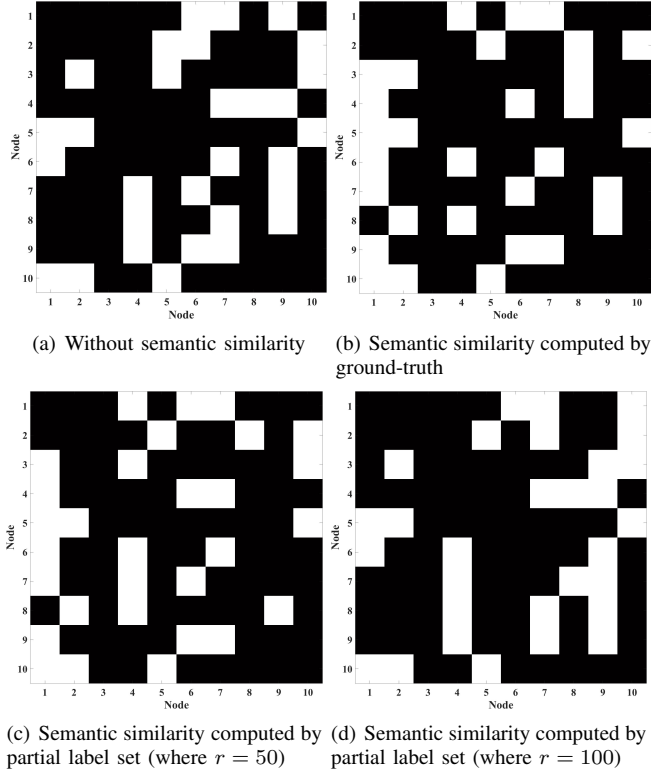
Fig. 10. An example of the constructed feature graphs with/without semantic information and under different noise densities, where the number of nearest neighbors is set as 3.
