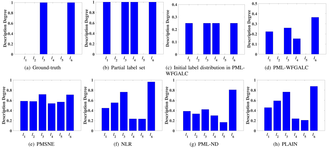
Fig. 8. An example of label distributions or label confidences learned by PML-WFGALC and other methods on the Emotions dataset.
