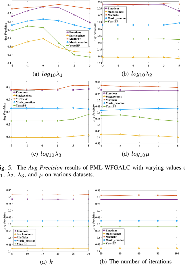
Fig. 6. The Avg Precision results of PML-WFGALC with varying values of k and the number of iterations on various datasets.
