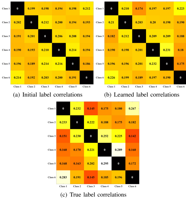
Fig. 11. An example of the learned label correlations.
