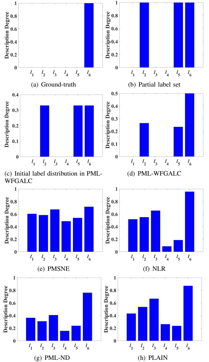
Fig. 9. The second example of label distributions or label confidences learned by PML-WFGALC and other methods on the Emotions dataset.
